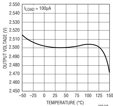
Output Voltage LT3008-2.5
