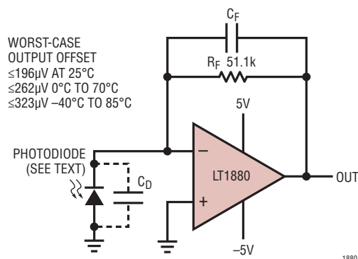
Figure 3. Precision Photodiode Amplifier
