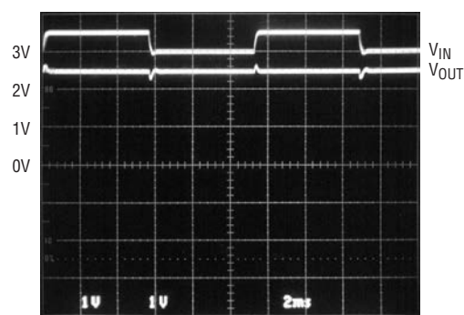
Figure 2. Output Response to 0.5V Ripple on V_{\text{IN}}
