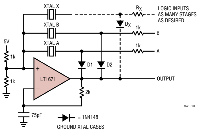
Figure 8. Switchable Output Crystal Oscillator. Biasing A or B High Places Associated Crystal in Feedback Path. Additional Crystal Branches Are Permissible
