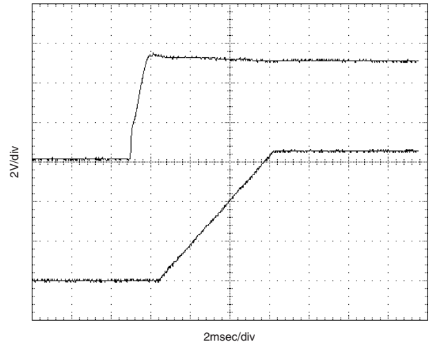
Power-Up From V IN
