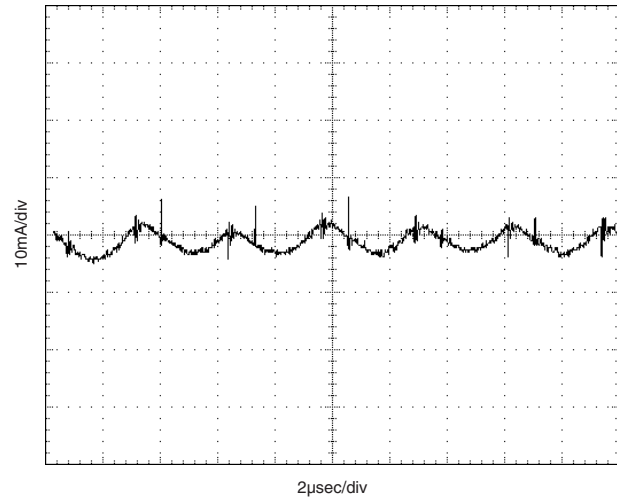
Input Reflected Ripple Current
