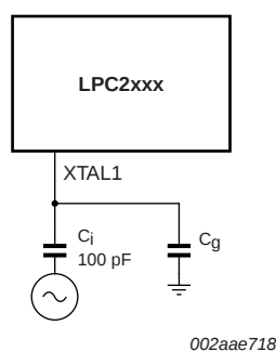
Fig 27. Slave mode operation of the on-chip oscillator
