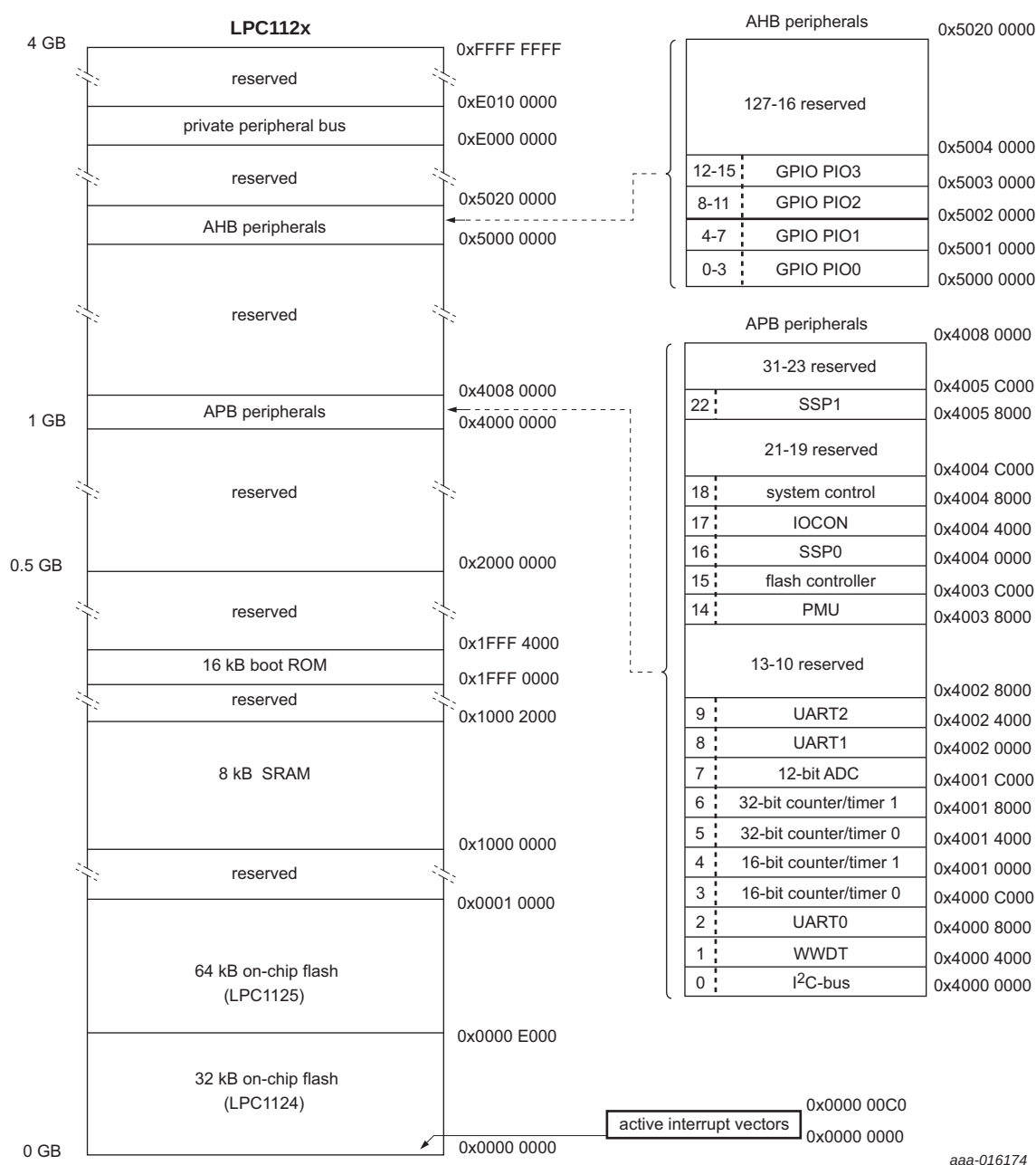
Fig 3. LPC112x memory map
