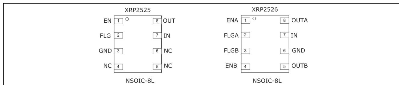
Fig. 3: XRP2525 - XRP2526 Pin Assignment
