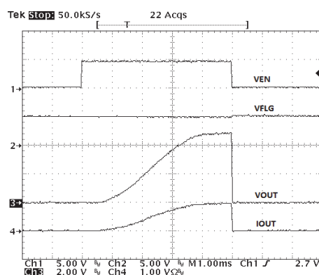
Fig. 25: Turn-On, Turn-Off Characteristics (XRP2526-1) COU = 1uF, Rload = 5.1Ω
