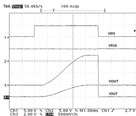
Fig. 24: Turn-On, Turn-Off Characteristics (XRP2526-1) COU = 1uF, Rload = 10Ω
