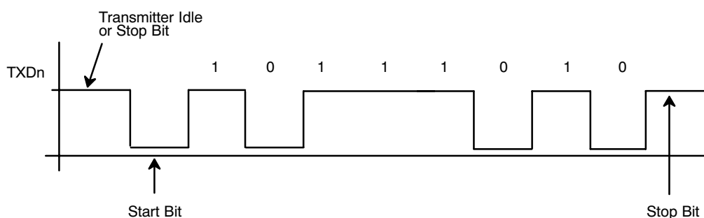
Figure 17. The Output Waveform of the Transmitter while sending 5D 16 (8-N-1 protocol).
