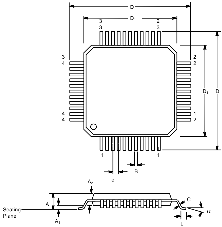
44 LEAD LOW-PROFILE QUAD FLAT PACK (LQFP)
