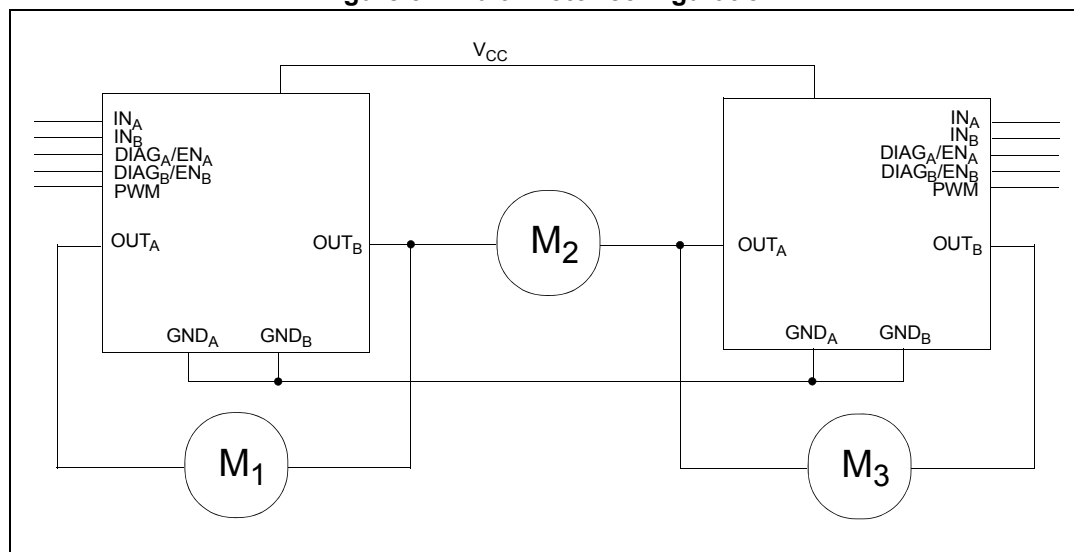
Figure 34. Multi-motor configuration
