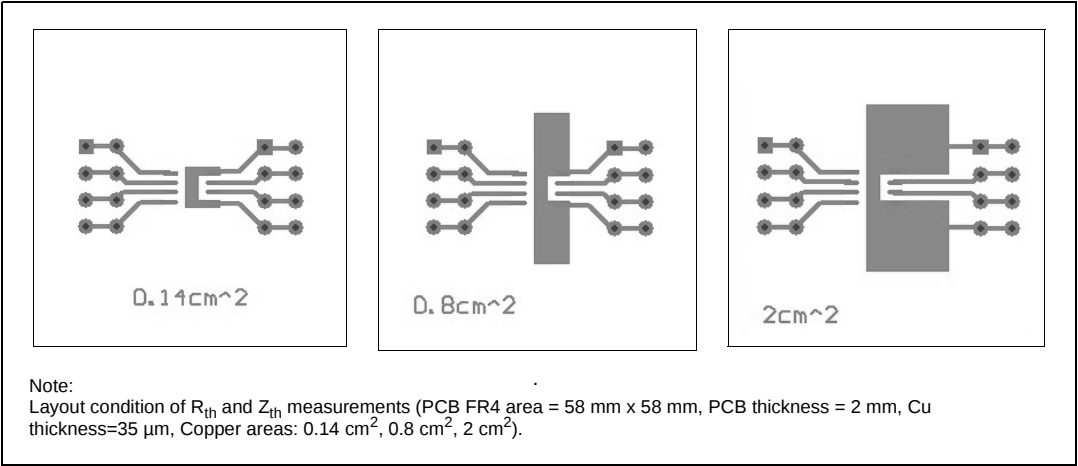
Figure 27. PC board
