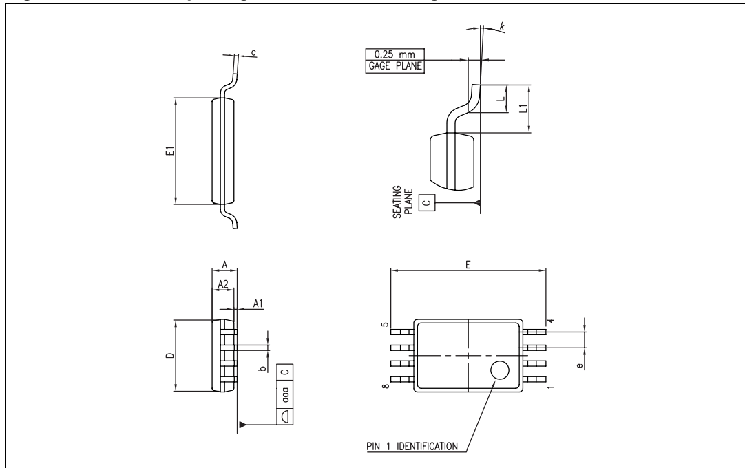
Figure 40. TSSOP8 package mechanical drawing
