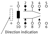
1 coil latching (Reset)
