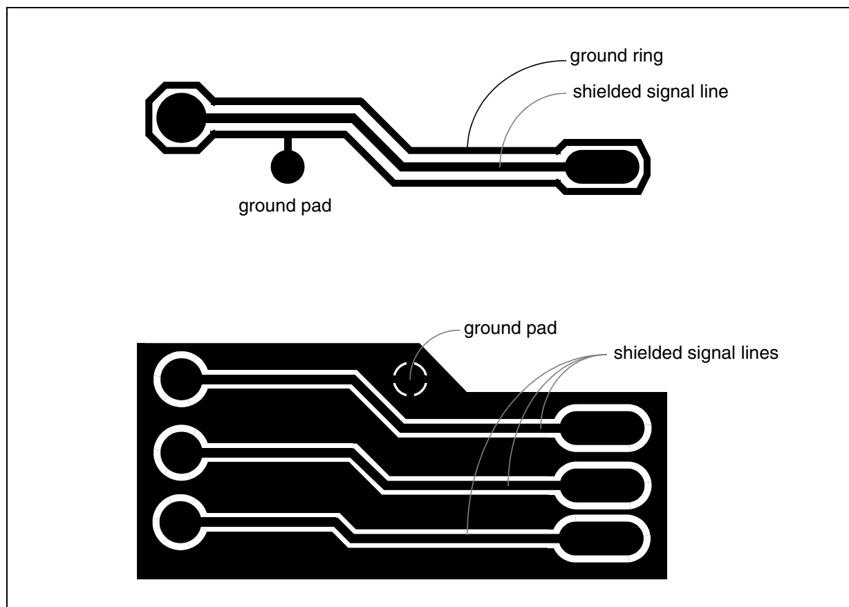
Figure 6-20. Shielding signals
