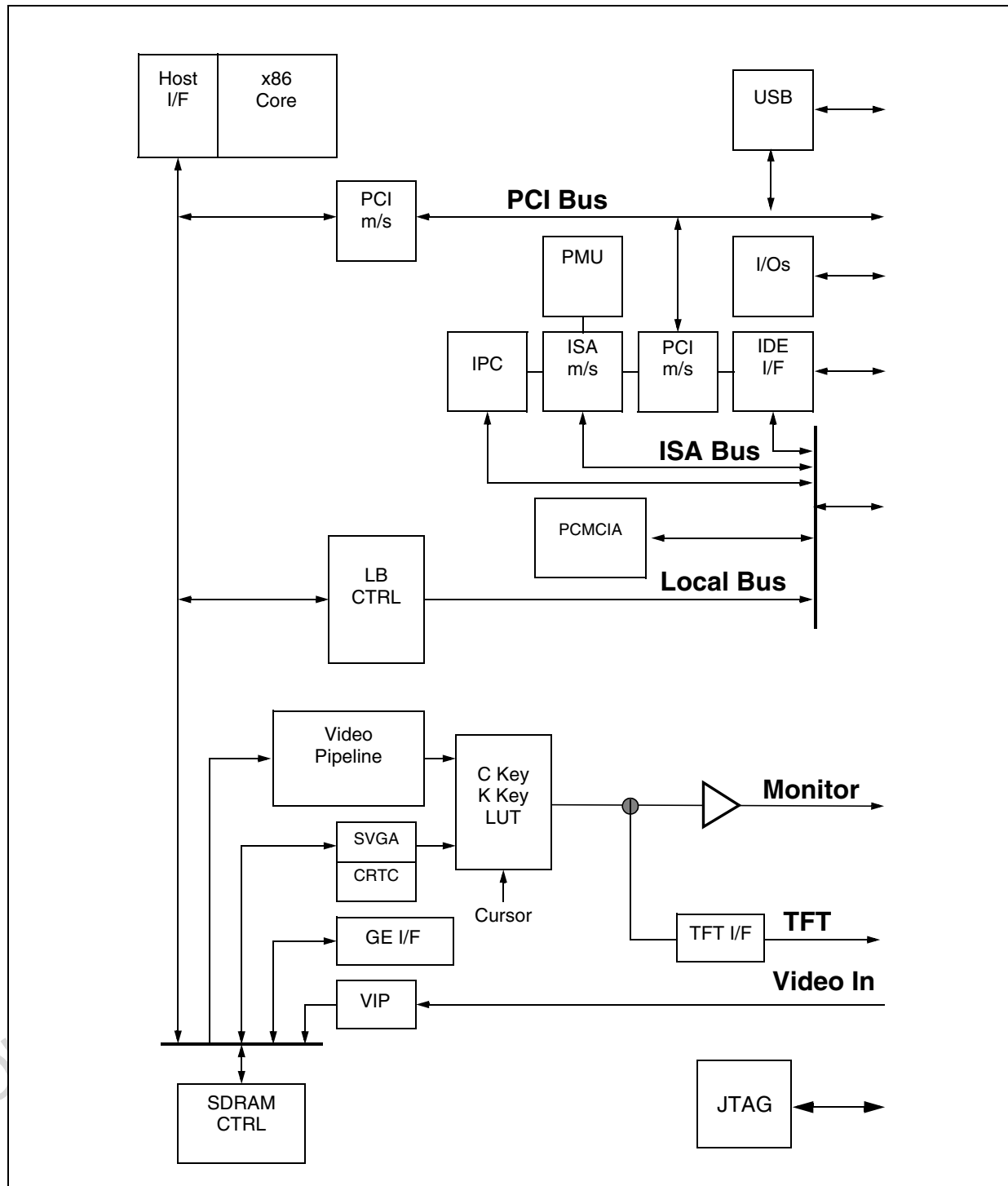
Figure 1-1. Functional description.
