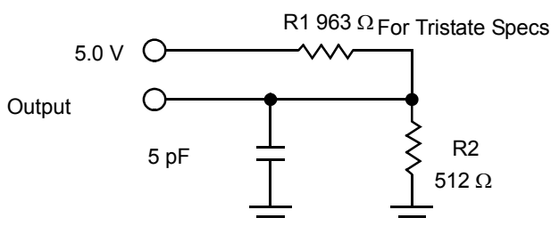
Figure 7. AC Test Loads
