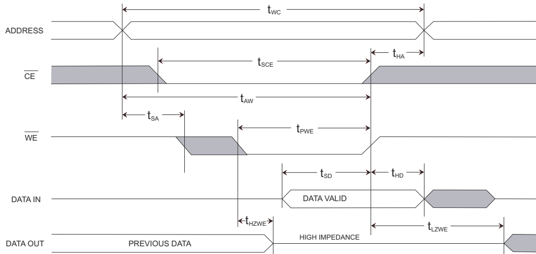
Figure 11. SRAM Write Cycle 2: \overline{CE} Controlled [13, 14]
