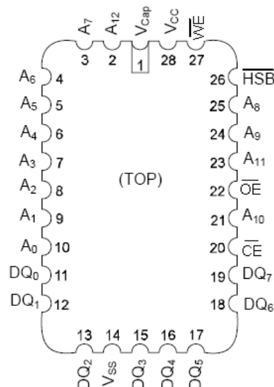
Figure 2. Pin Diagram - 28-Pin LCC
