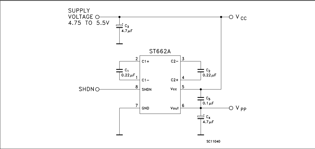
Figure 16. Electrical schematic
