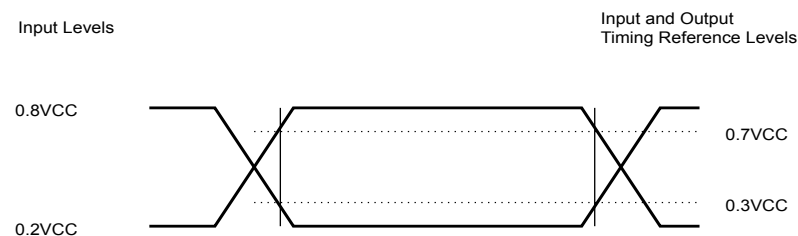
Figure 74. AC test measurement I/O waveform
