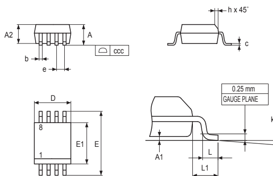
Figure 78. SO8N – Outline
