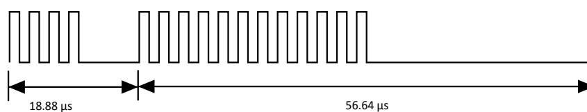
Figure 92. End of frame, high data rate, one subcarrier, fast commands
