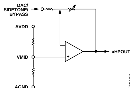
Figure 22. Headphone Output
