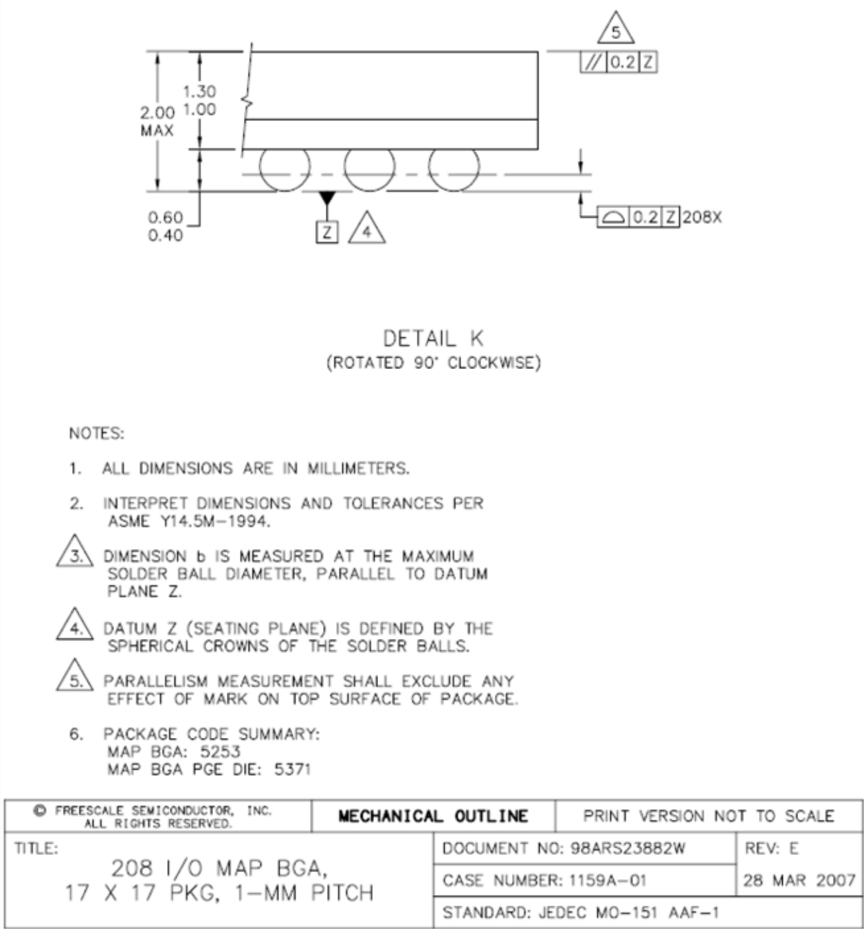
Figure 31. 208 MAPBGA Package Detail
