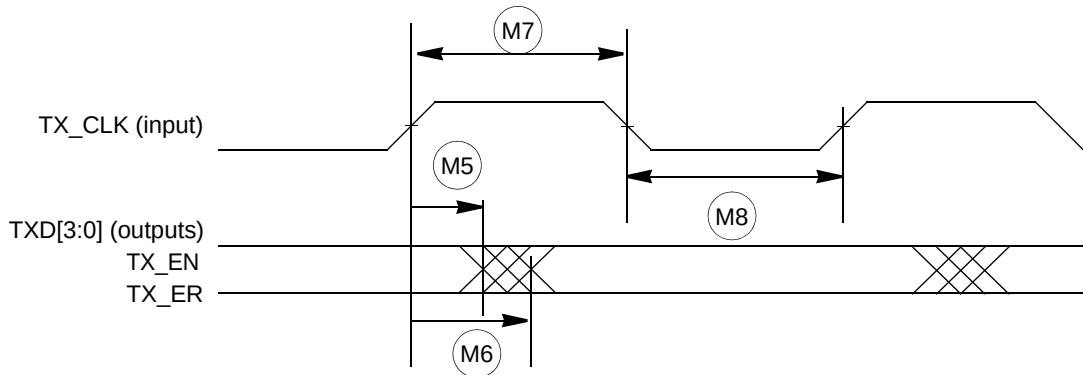
Figure 27. MII Transmit Signal Timing Diagram
