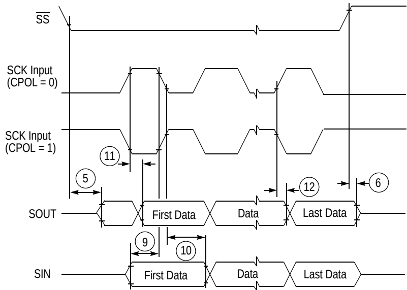
Figure 19. DSPI Classic SPI Timing — Slave, CPHA = 1
