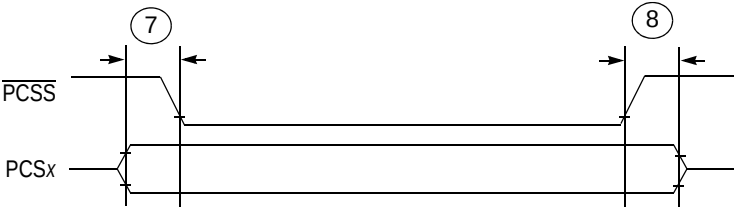
Figure 24. DSPI PCS Strobe (PCSS) Timing
