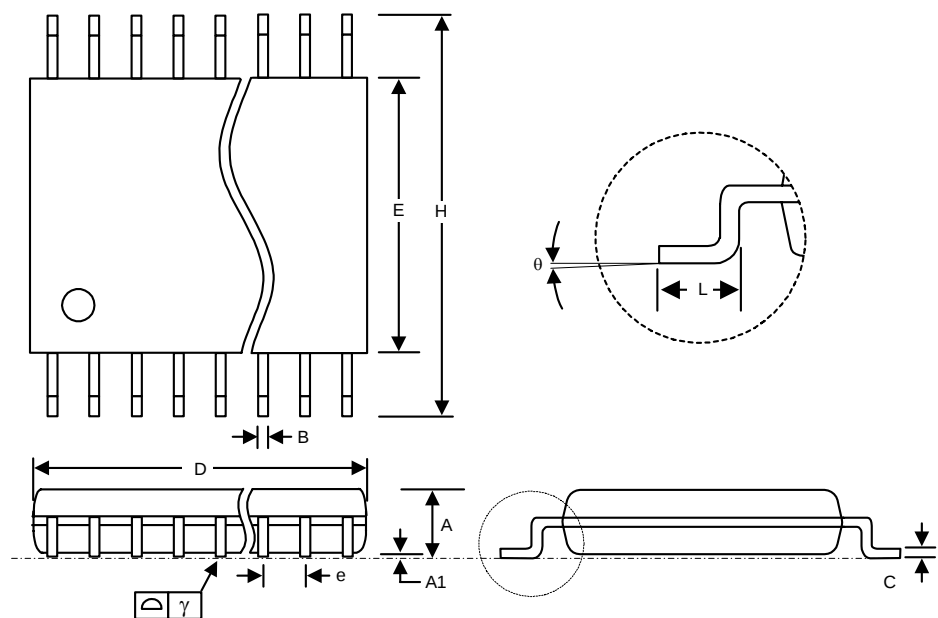
Figure 8. 24-Pin Thin Shrink Small Outline Package (TSSOP)
