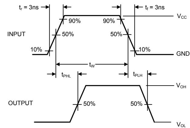
Figure 2. AC Waveforms
