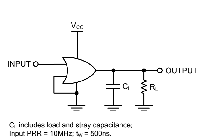
Figure 1. AC Test Circuit
