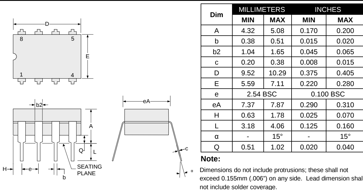
Figure 2 • Y 8-Pin CERPDP Package Dimensions
