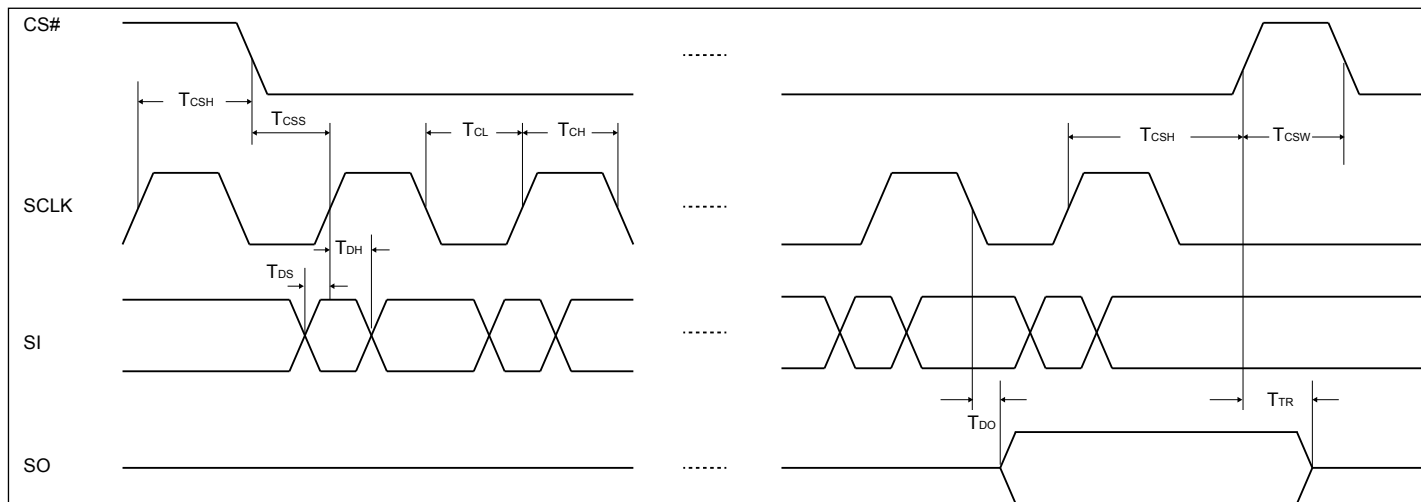
Figure 9. SPI-bus Timing
