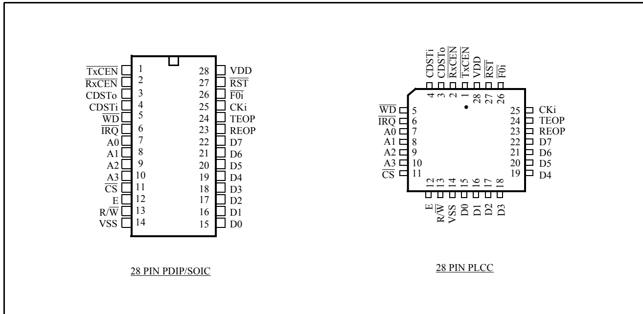
Figure 2 - Pin Connections
