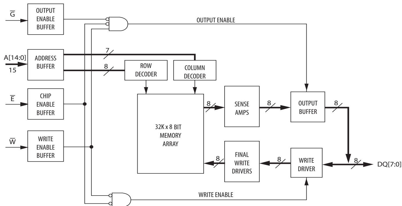
Figure 1.1 Block Diagram
