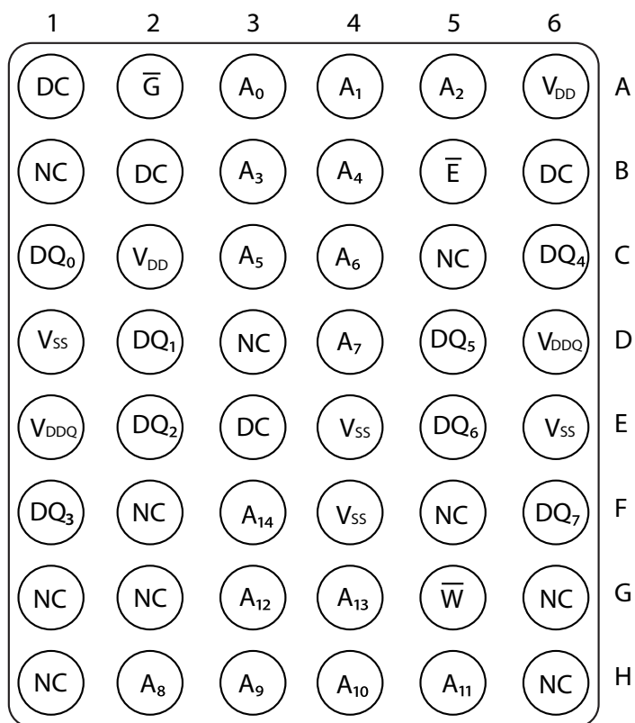
48 Pin FBGA
