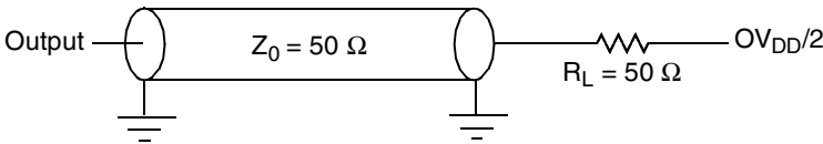
Figure 29. GPIO AC Test Load
