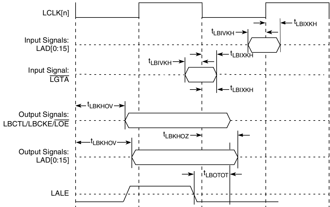
Figure 15. Local Bus Signals, Nonspecial Signals Only
