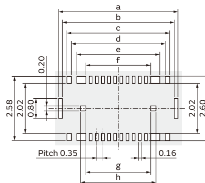
MLF14/MLF20 Plug Receptacle (Below is MLF20 plug receptacle for reference.)
