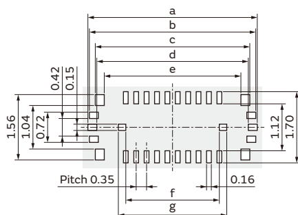
MLF14/MLF20 Receptacle (Below is MLF20 receptacle for reference.)
