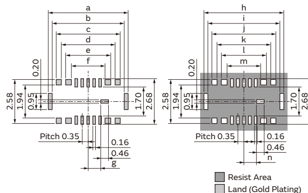
Plug Receptacle
