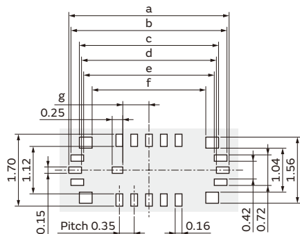
MLF06/MLF10 Receptacle (Below is MLF10 receptacle for reference.)
