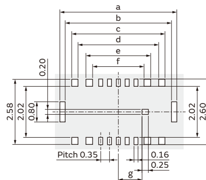
MLF06/MLF10 Plug Receptacle (Below is MLF10 plug receptacle for reference.)
