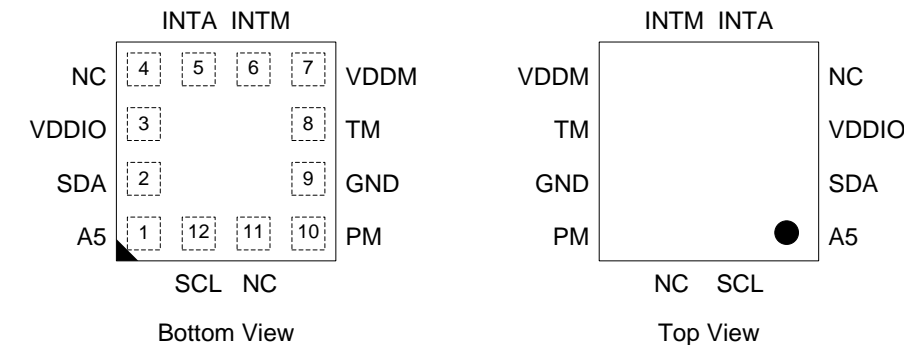
Figure 5. Package Pins
