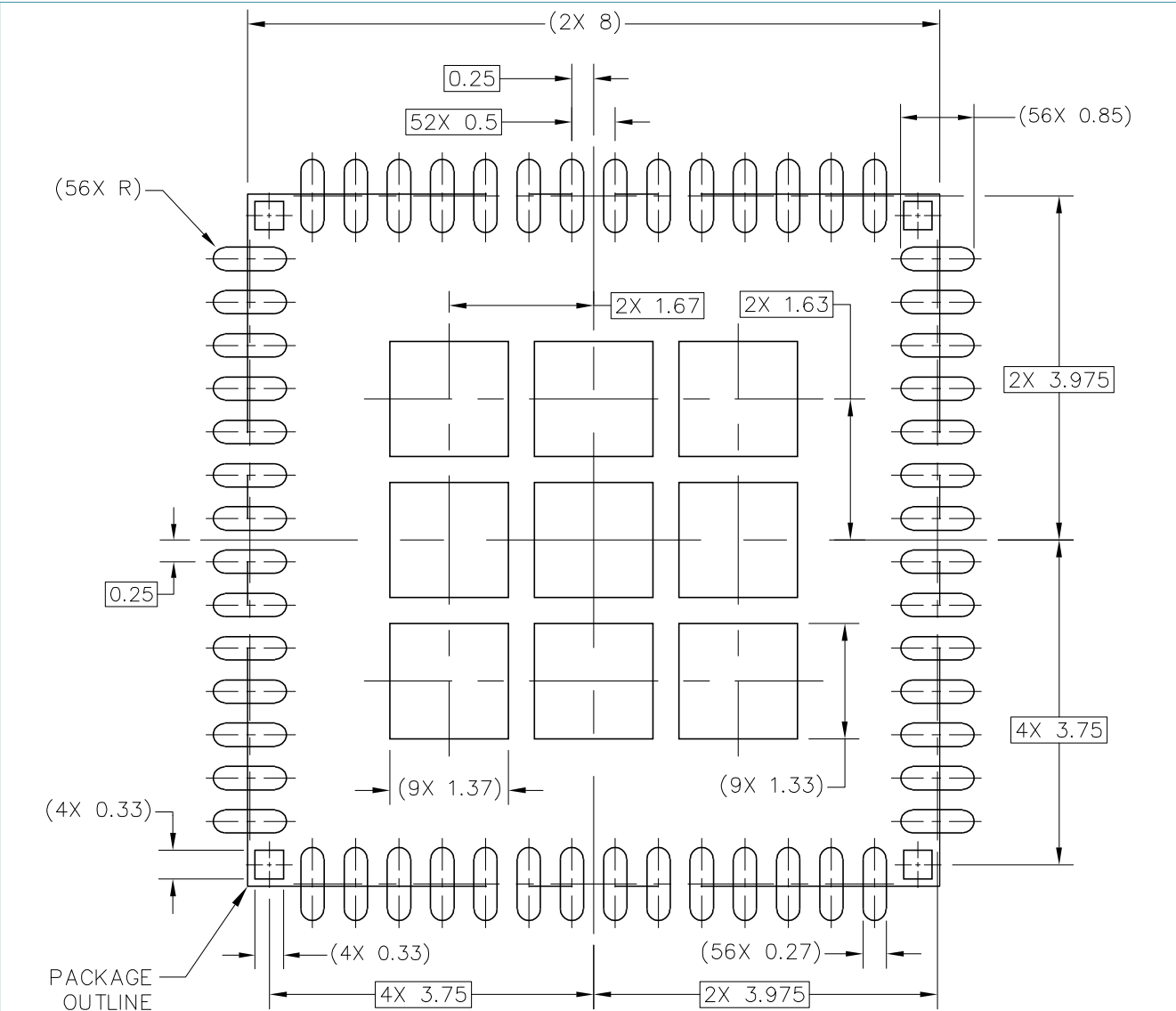
Figure 52. Solder paste stencil for E-type HVQFN56
