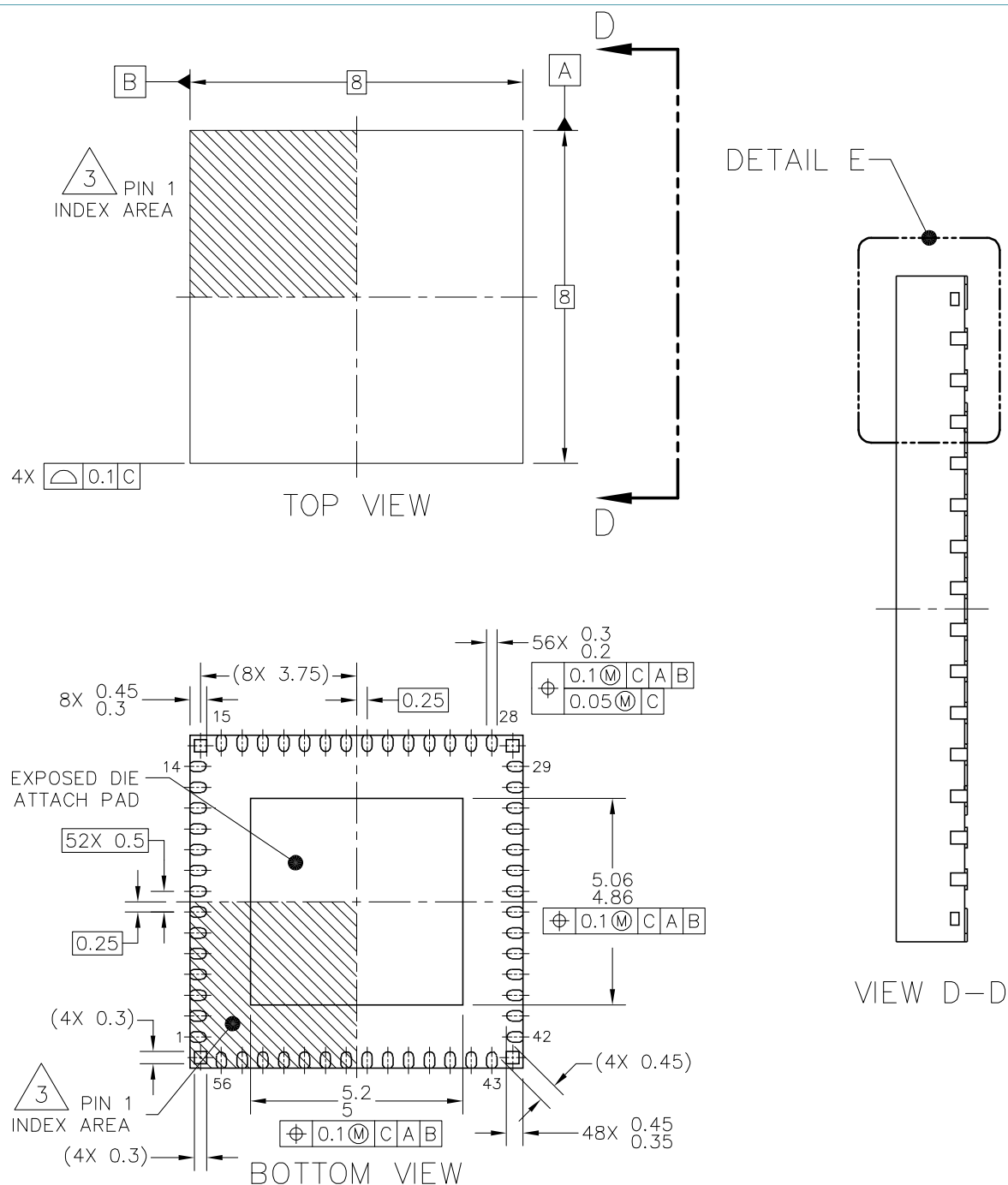
Figure 42. Package outline for E-type HVQFN56
