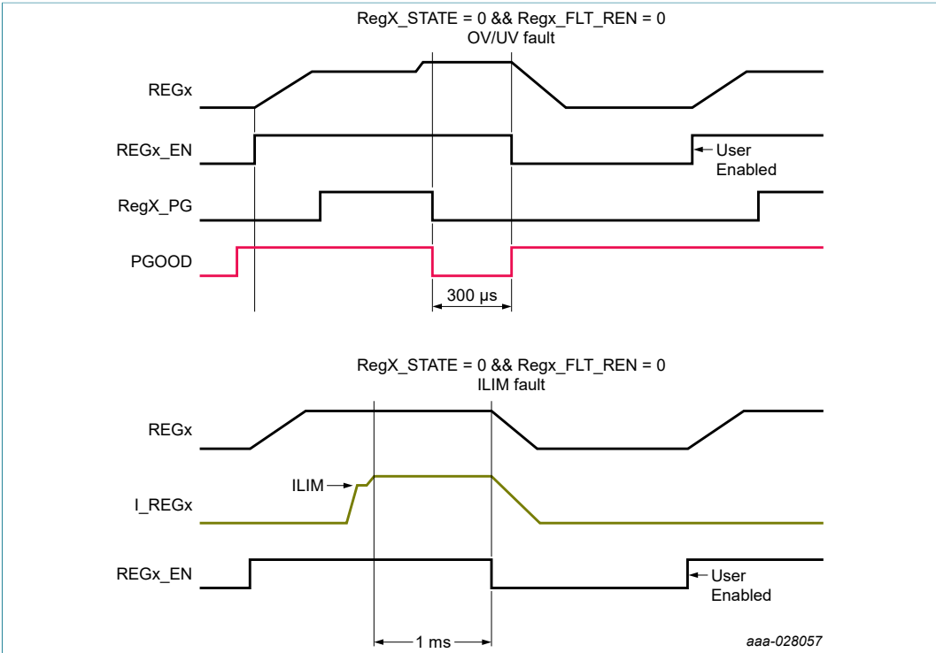
Figure 12. Regulator turned off with RegX_STATE = 0 and FLT_REN = 0
