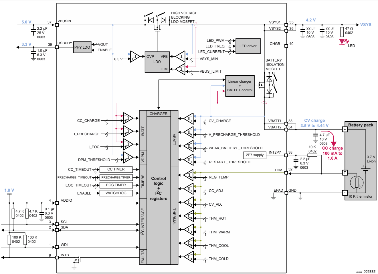
Figure 12. Battery charger internal block diagram
