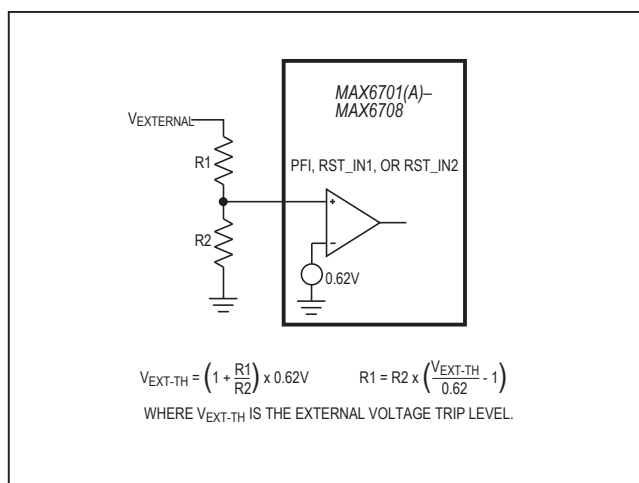
Figure 8. Calculating Adjustable Voltage Thresholds
