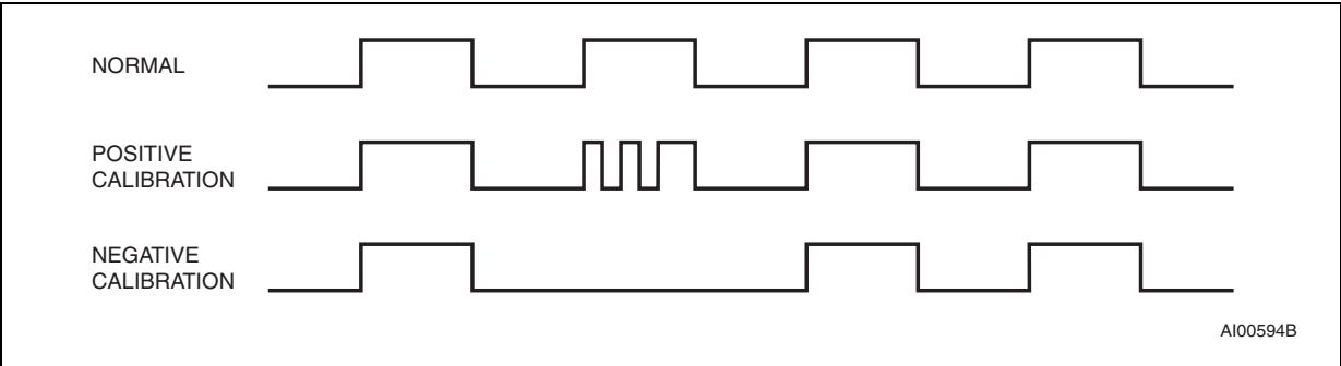
Figure 9. Clock calibration
