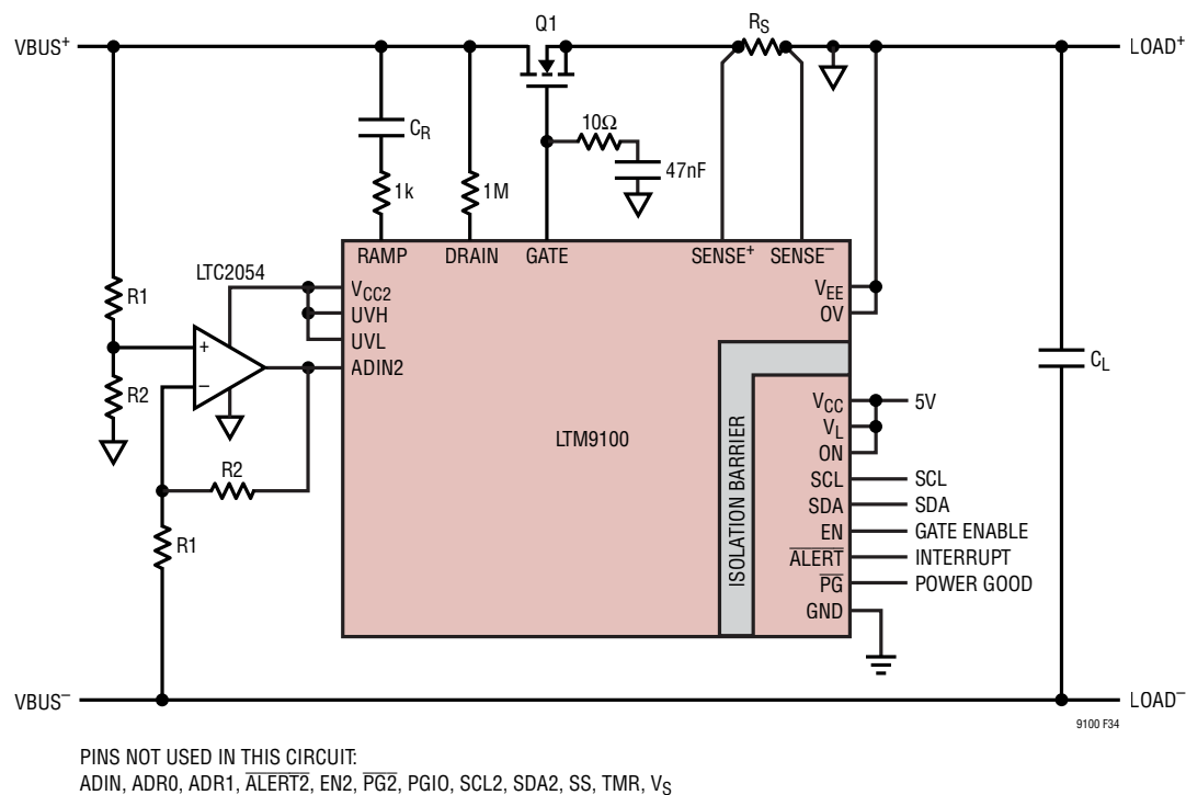
Figure 34. High Side Inrush Current Control with Line/Load Voltage Sense
