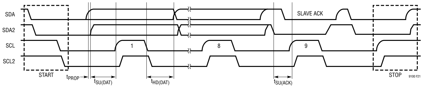
Figure 21. I²C Timing Diagram
