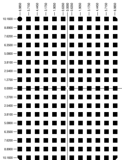
SUGGESTED PCB LAYOUT TOP VIEW
