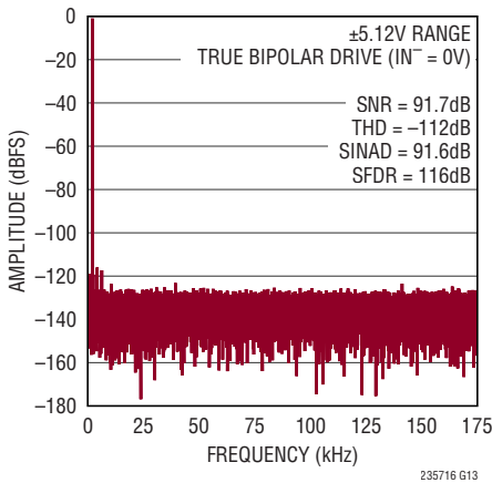
32k Point FFT f_{SMPL} = 350\text{ksps} , f_{IN} = 2\text{kHz}
