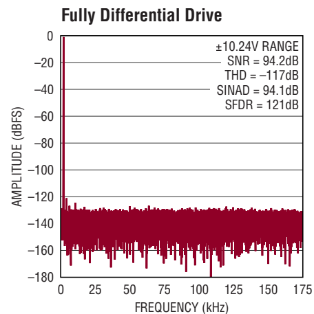
Figure 6c. IN^+/IN^- = -1\text{dBFS} 2kHz Fully Differential Sine, V_{\text{CM}} = 0\text{V} , 32k Point FFT, f_{\text{SAMPL}} = 350\text{kps} . Circuit Shown in Figure 6a
