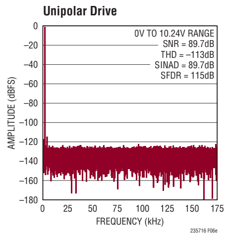
Figure 6e. IN^+ = -1\text{dBFS} 2kHz Unipolar Sine, IN^- = 0\text{V} , 32k Point FFT, f_{\text{SAMPL}} = 350\text{kps} . Circuit Shown in Figure 6a
