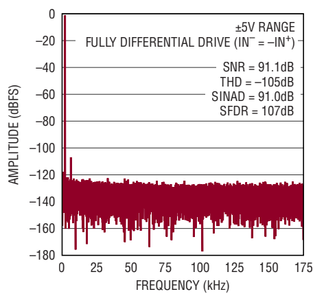
Figure 7c. IN + /IN - = 450mV 200Hz Fully Differential Sine, 0\text{V} \leq V_{\text{CM}} \leq 24\text{V} , 32k Point FFT, f_{\text{SMPL}} = 350\text{ksps} . Circuit Shown in Figure 7a
