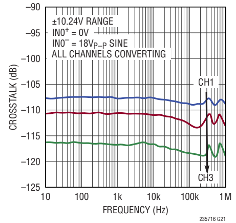
Crosstalk vs Input Frequency and Channel
