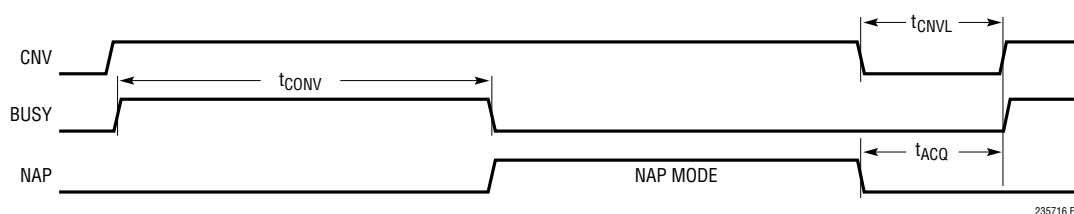
Figure 13. Nap Mode Timing for the LTC2357-16
