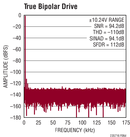
Figure 6d. IN^+ = -1\text{dBFS} 2kHz True Bipolar Sine, IN^- = 0\text{V} , 32k Point FFT, f_{\text{SAMPL}} = 350\text{kps} . Circuit Shown in Figure 6a
