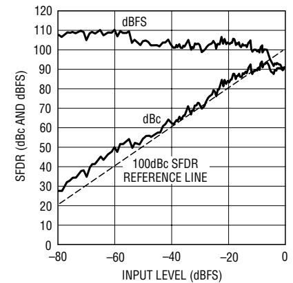
SFDR vs Input Level, f_{IN} = 70\text{MHz} , 2V Range, 80MSPs
