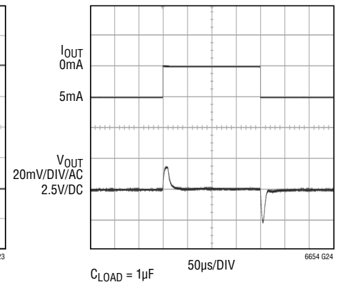
2.5V Load Transient Response (Sourcing)
