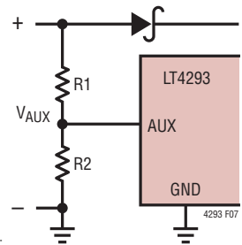
Figure 7. AUX Threshold and Hysteresis Calculation
