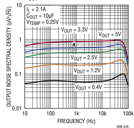
Output Noise Spectral Density, C_{SET} = 0
