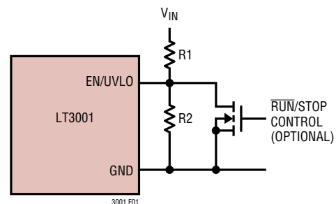
Figure 1. Undervoltage Lockout (UVLO)
