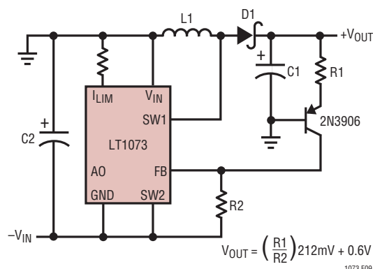
Figure 9. Negative-to-Positive Converter
