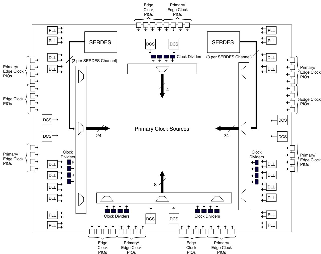
Figure 2-5. Clock Sources
