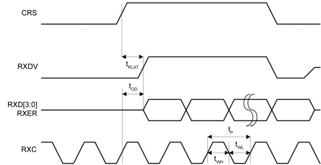
Figure 15. MII Receive Timing (10Base-T)
