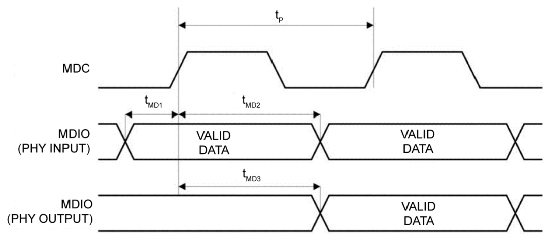
Figure 19. MDC/MDIO Timing
