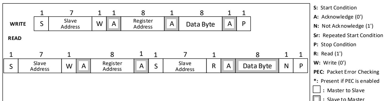
Figure 24: I2C Format
