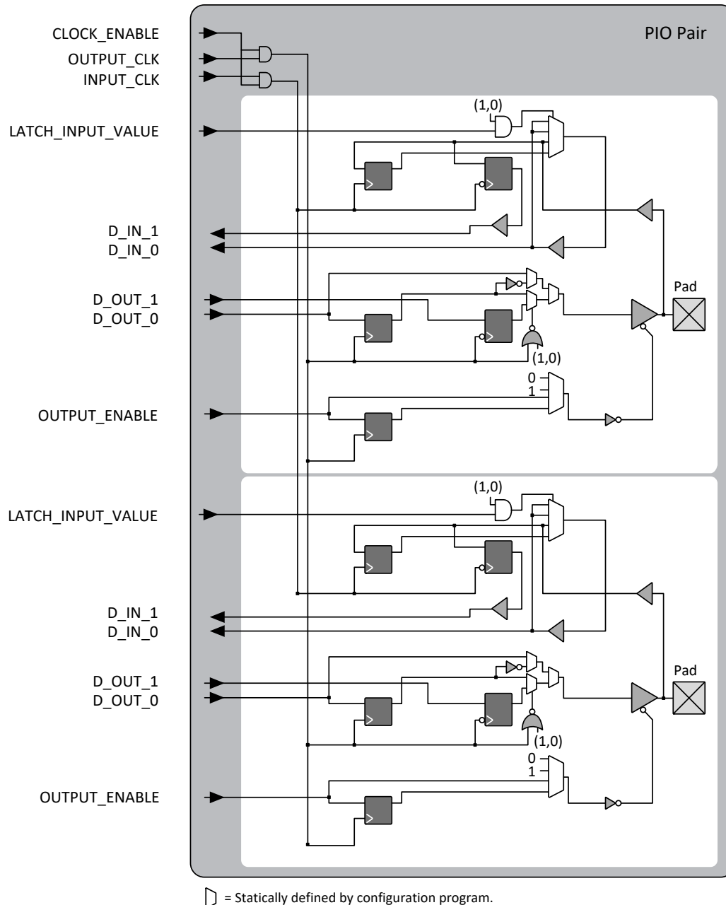
Figure 3.6. iCE40 I/O Register Block Diagram
