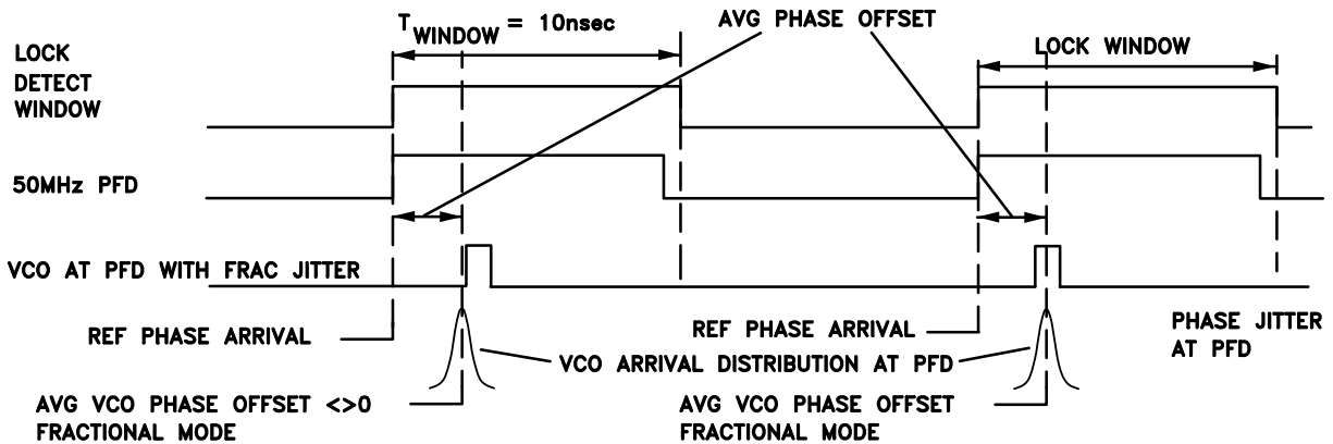
Figure 34. Lock Detect Window - Fractional Mode with Offset
