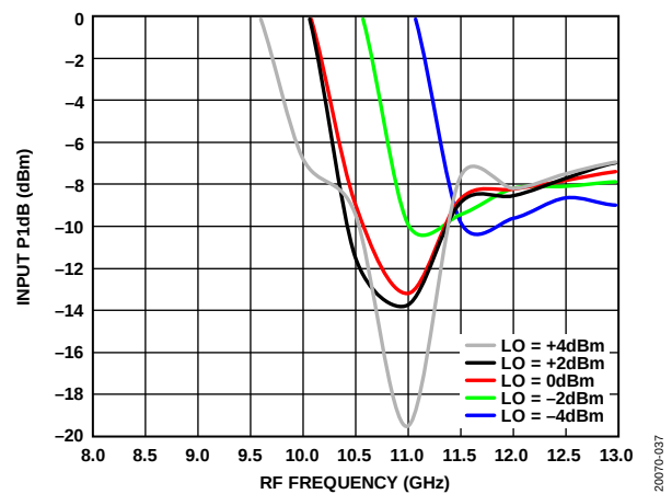
Figure 38. Input P1dB vs. RF Frequency at Various LO Powers, T_A = 25^\circ\text{C}
