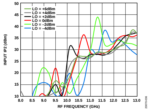
Figure 37. Input IP2 vs. RF Frequency at Various LO Powers, T_A = 25^\circ\text{C}
