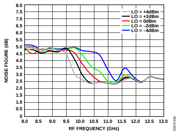
Figure 39. Noise Figure vs. RF Frequency at Various LO Powers, T_A = 25^\circ\text{C}
