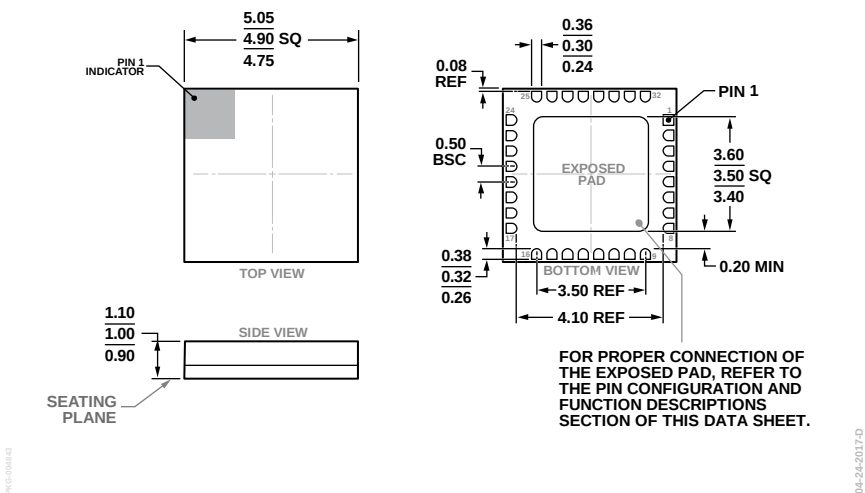
Figure 84. 32-Terminal Ceramic Leadless Chip Carrier (LCC) (E-32-1) Dimensions shown in millimeters
