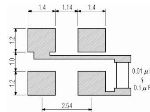
Figure 2) Land Pattern
